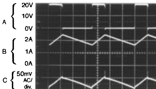
A: Output Pin Voltage, 10V/div. B: Inductor Current 1A/div. C: Output Ripple Voltage, 50 mV/div. Figure 20. Horizontal Time Base: 2 \mu\text{s} /div.
